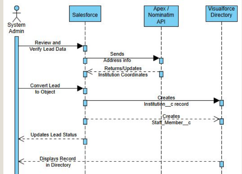
System Admin Sequence
